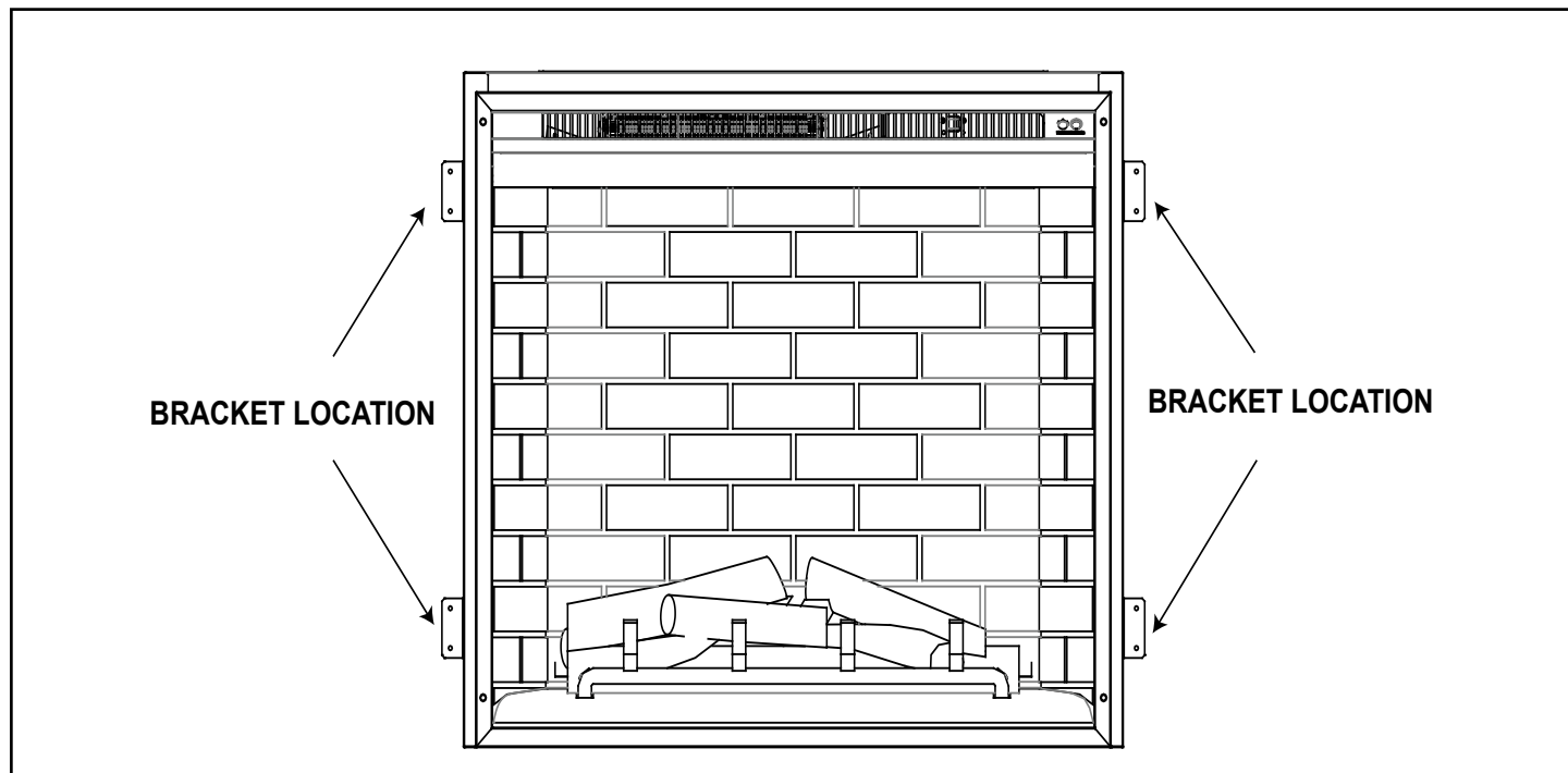
Figure 4.3 Bracket Locations
