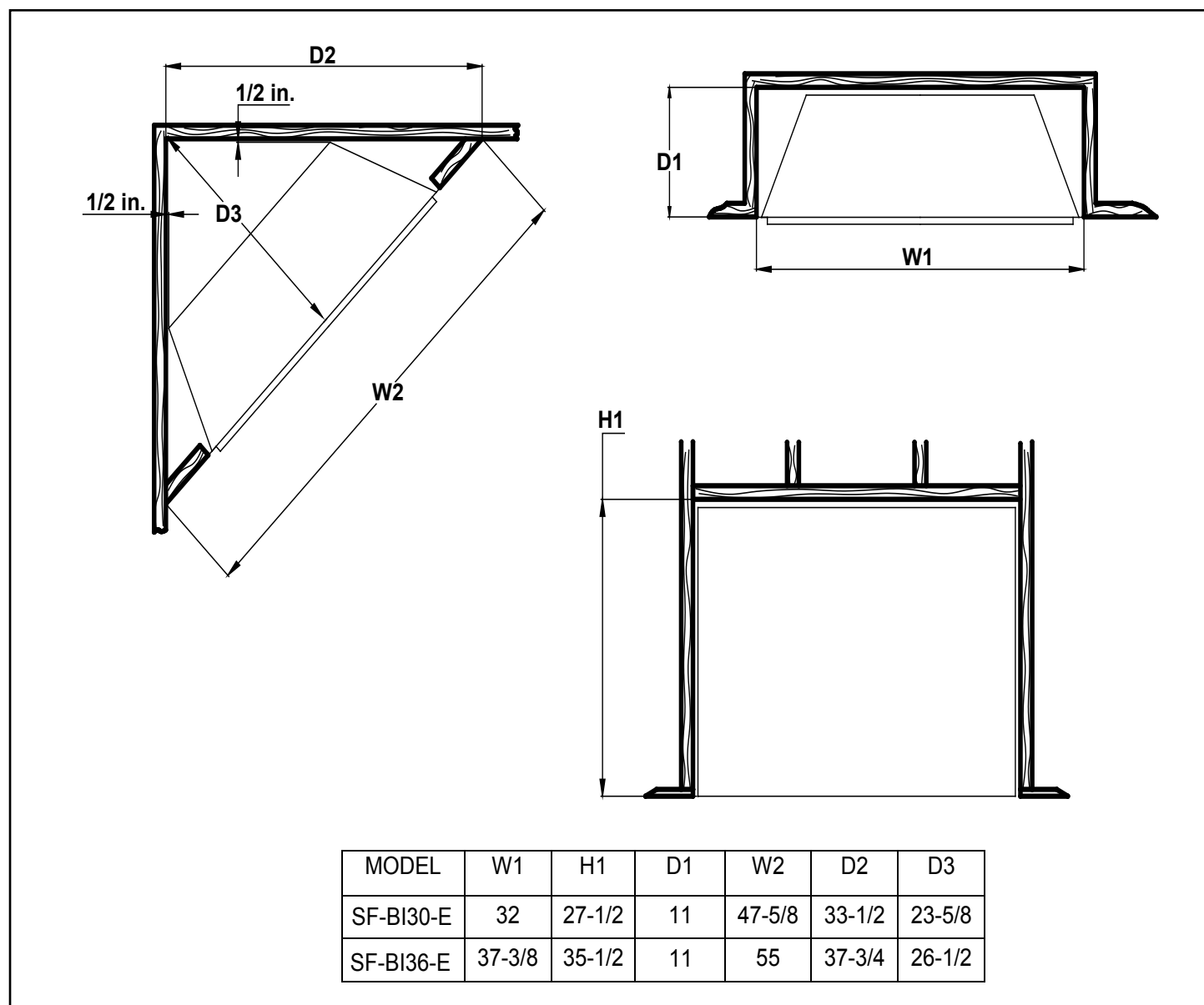
Figure 4.1 Clearance Requirements
