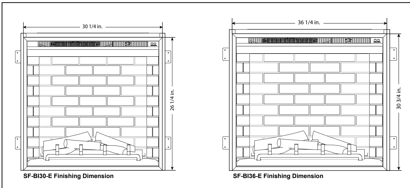
Figure 4.4 Finishing Dimensions
