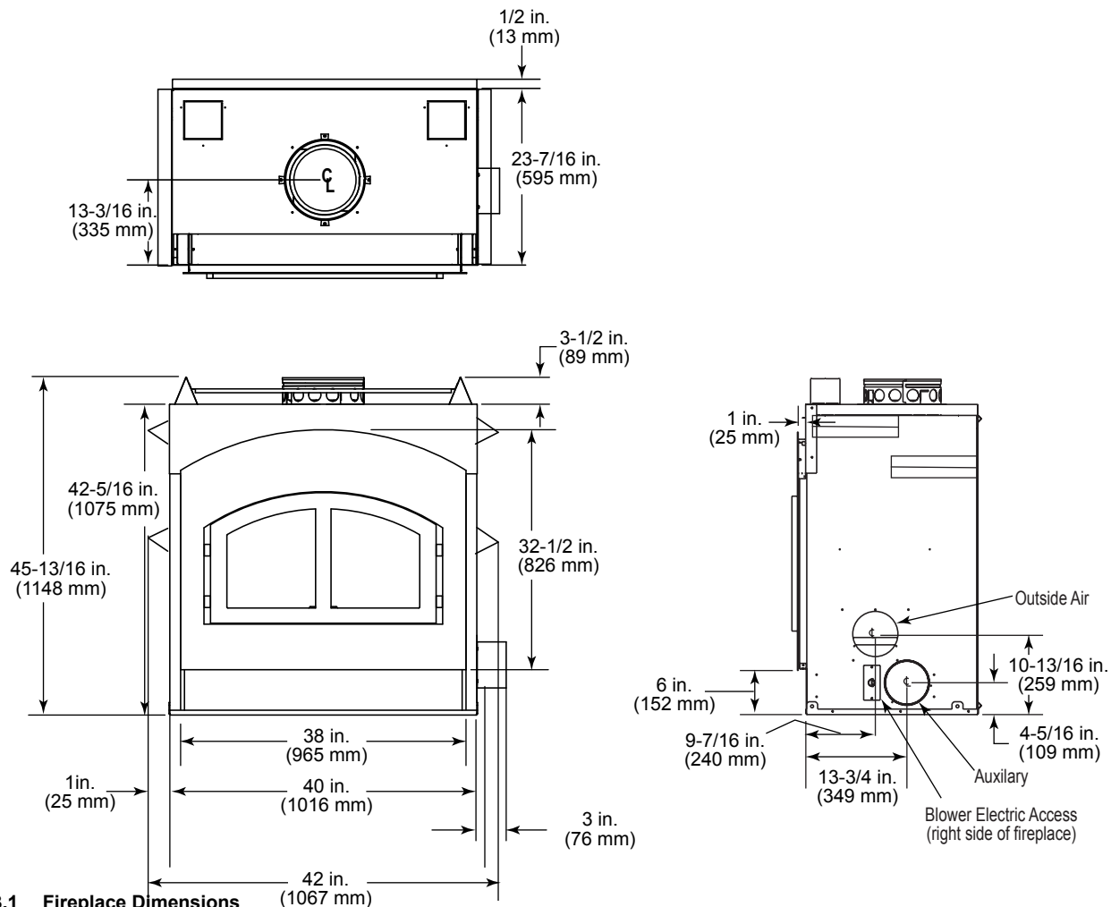
Figure 3.1 Fireplace Dimensions
