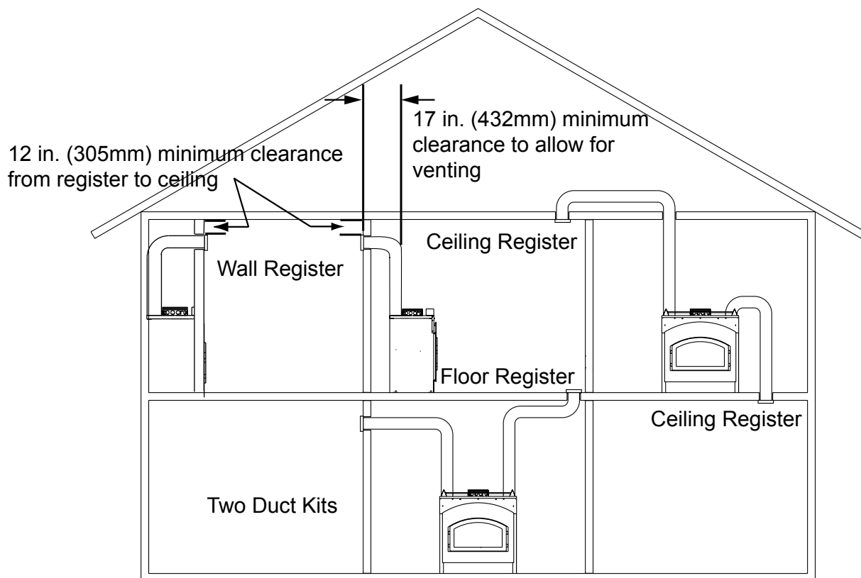
Figure 3.15 Minimum Clearances to Combustibles
