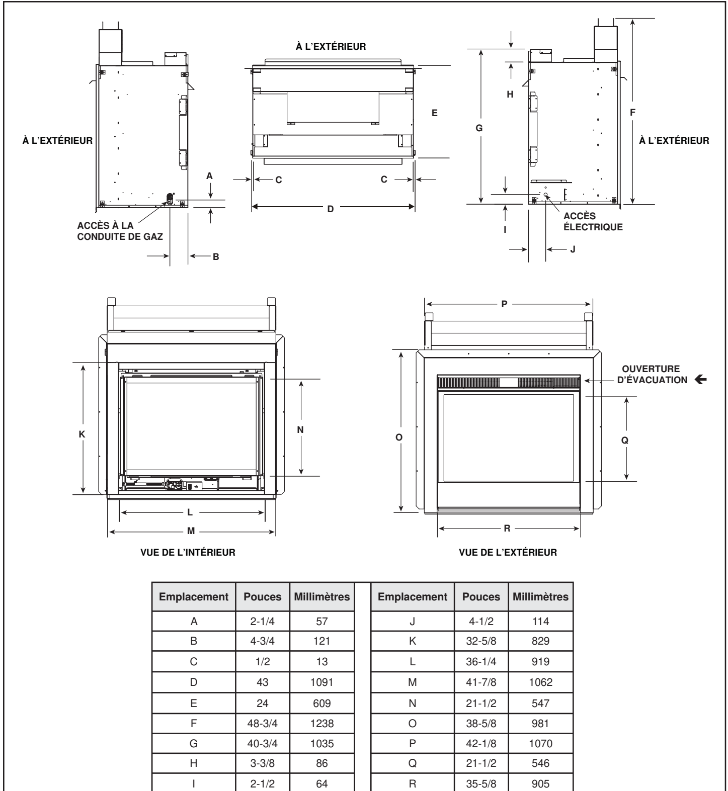
Figure 13.1 Dimensions du foyer
