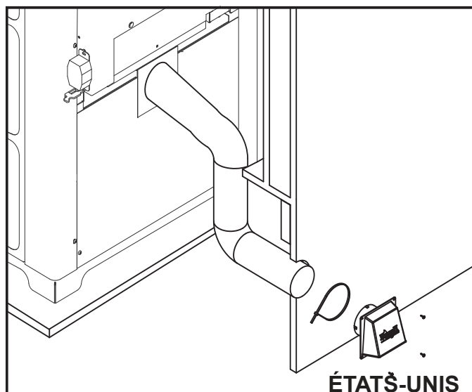
Figure 15.2 - Installation au sol
