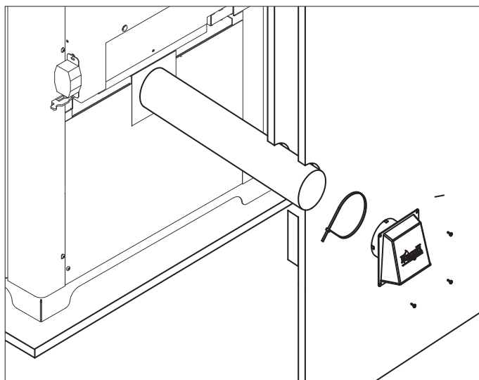
Figure 15.1 - Installation arrière
