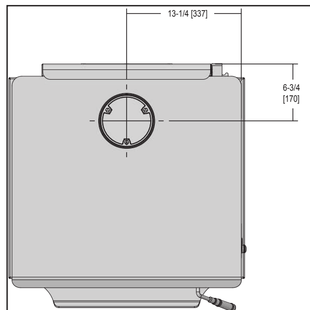
Figure 7.2 Top View
