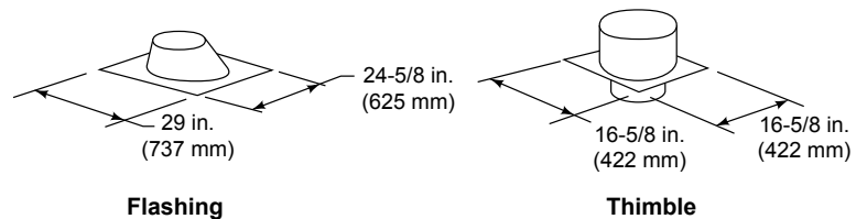
12966A Manufactured Home Thimble Kit
