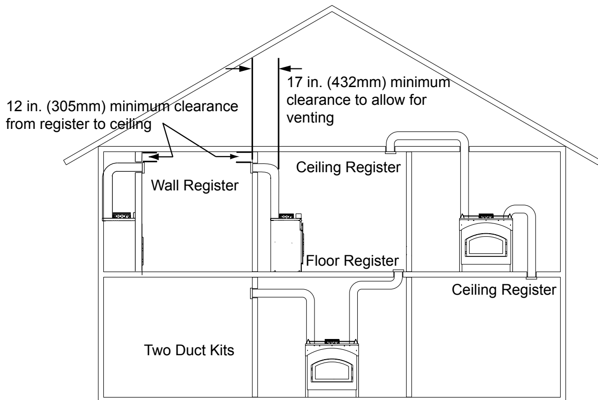
Figure 3.14 Minimum Clearances to Combustibles
