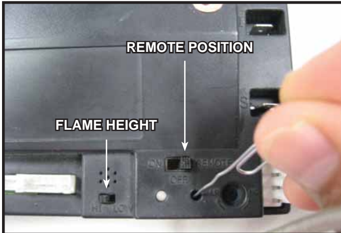
Figure 5. Programming RC100
