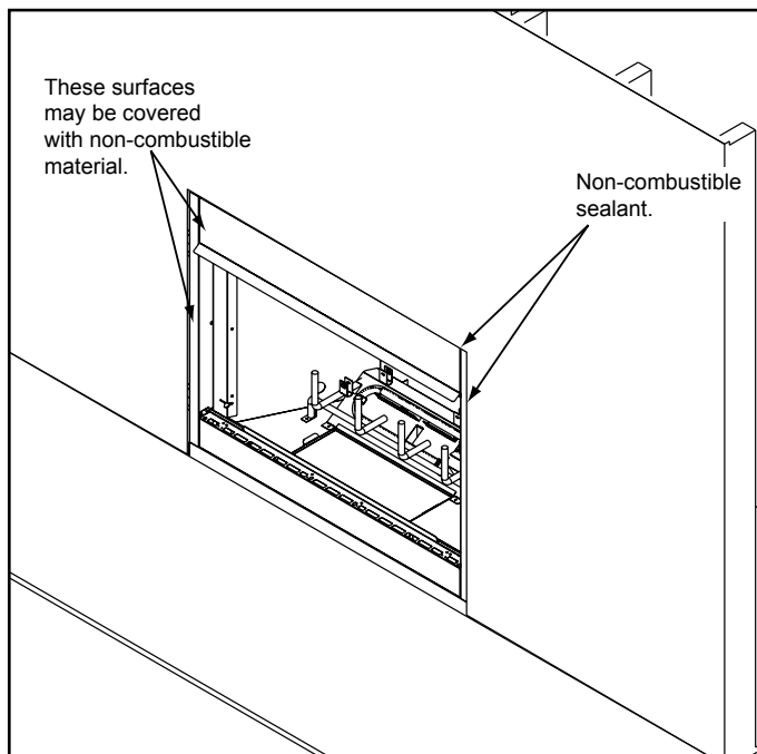
Figure 7.1 Non-combustible Facing
