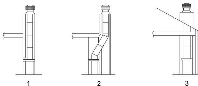
Figure 3.4 Chase Constructions
