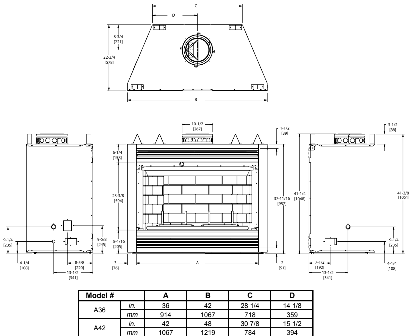
Figure 3.1 Fireplace Dimensions
