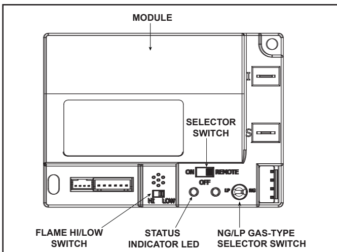
Figure 3.8 Control Module
