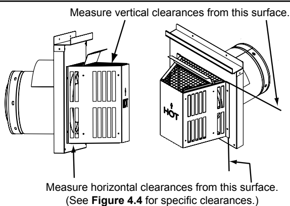
Figure 4.1 Termination Clearances
