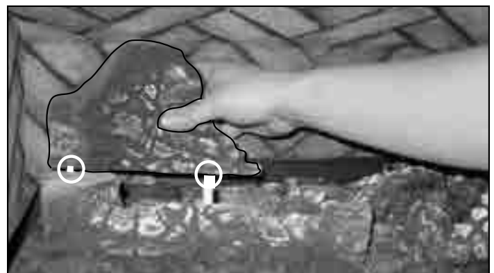
Figure 8.15 - Install the left rear log (#3) over the locator pins in the burner pan.
