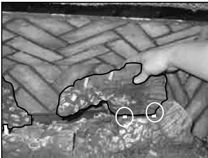
Figure 8.16 - Install the right rear log (#4) over the locator pins in the burner pan.
