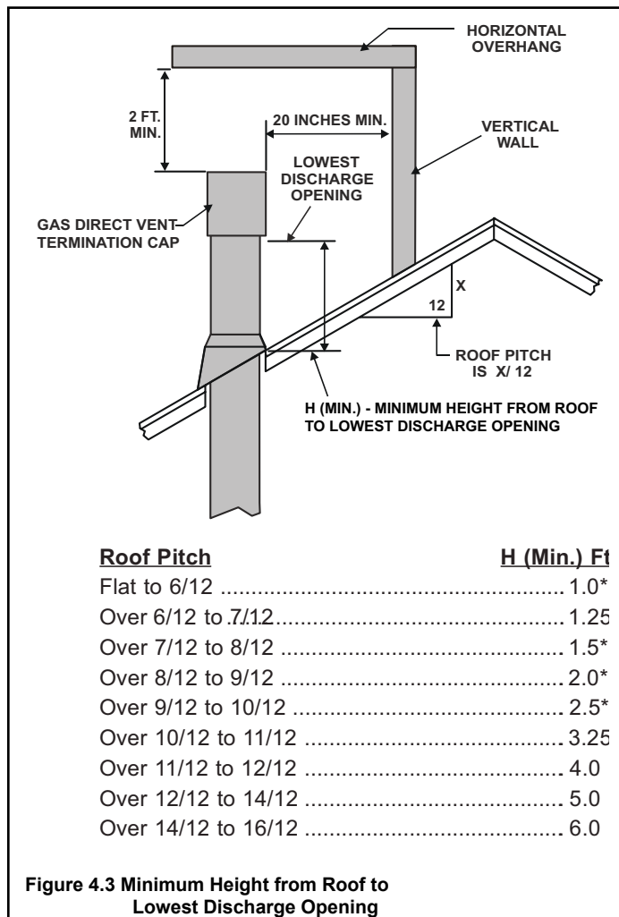
Figure 4.3 specifies minimum vent heights for various pitched roofs.
