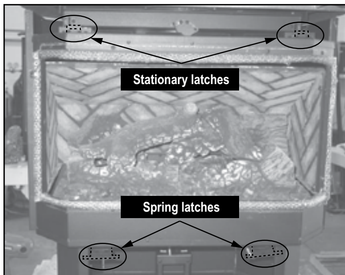
Figure 8.1 - Open lower access panel. Pull out and unhook the two spring latches on the bottom of the appliance that secure the door.
