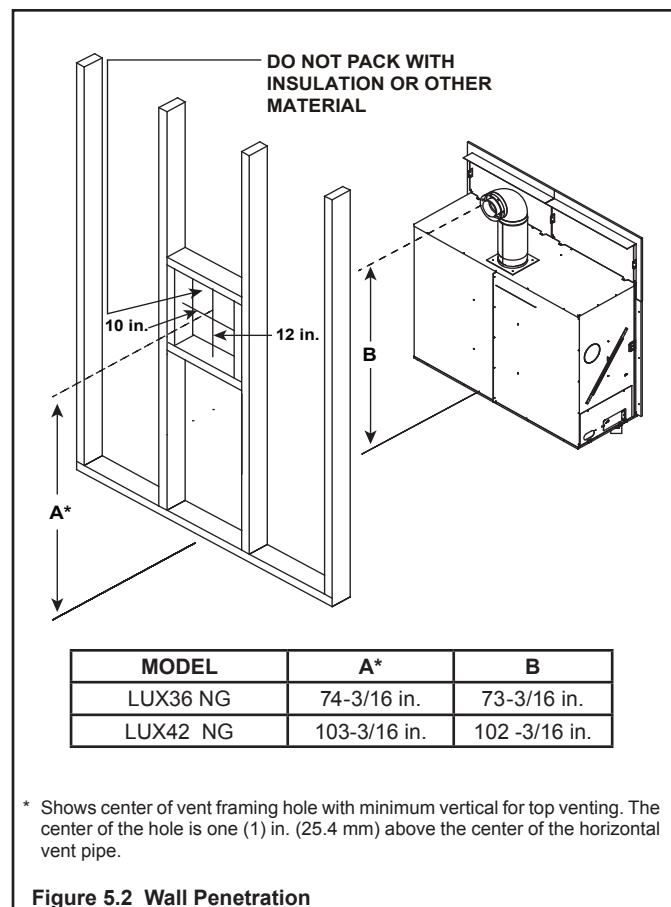
Figure 5.2 Wall Penetration
