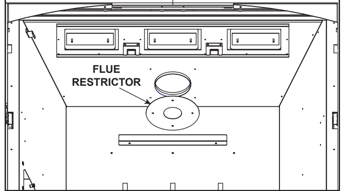
Figure 4.10 Flue Restrictor Installation
