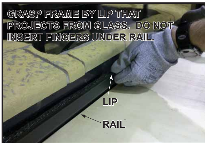
Figure 11.6. Install Glass
