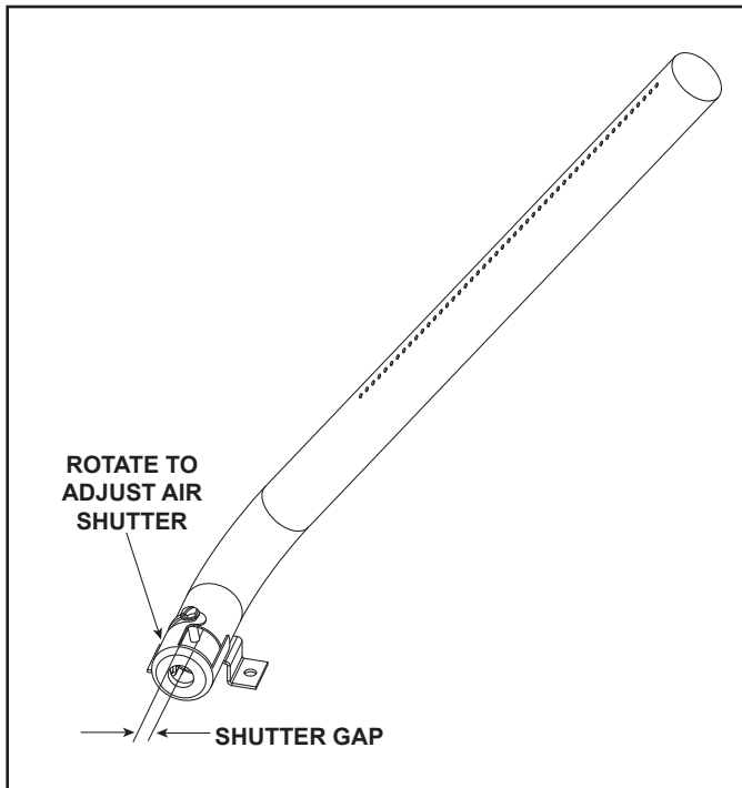
Figure 9.1 Air Shutter
