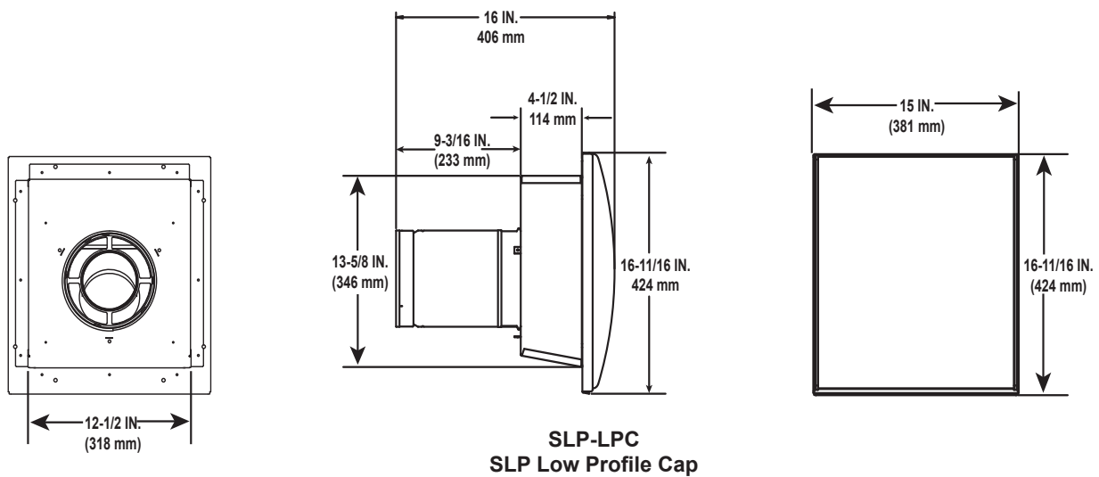
Figure 12.4 Vent Components
