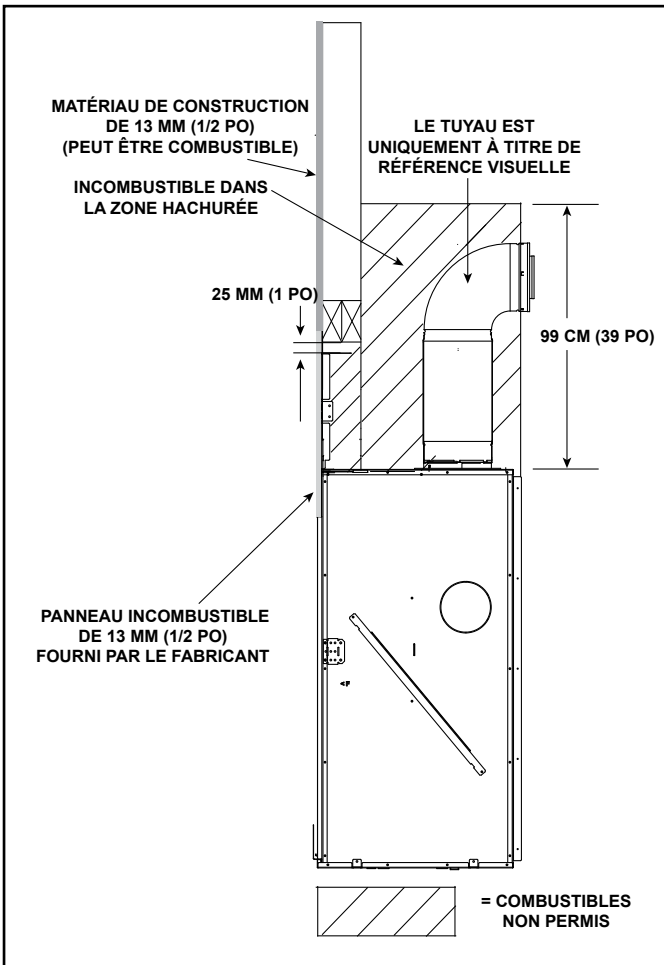
Figure 3.7 Zone incombustible
