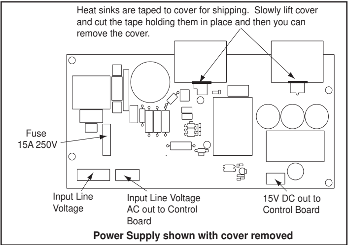
Figure 32.1 - Power Supply
