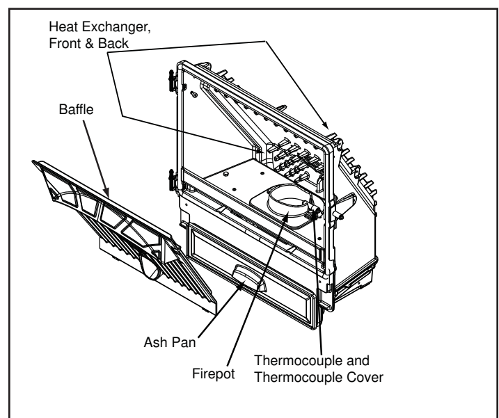
Figure 33.3 - Heat Exchanger, Baffle, Ash Pan, Firepot Thermocouple & Thermocouple Cover
