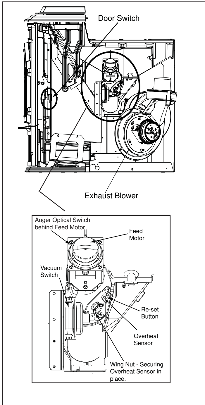
Figure 33.1 - Feed Motor, Vacuum Switch, Exhaust Blower, Overheat Sensor
