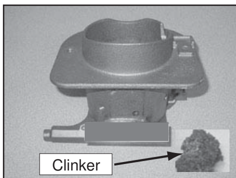
Figure 24.1 - Large Clinker
