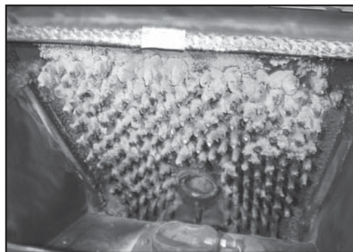
Figure 24.2 - Example of a dirty heat exchanger
