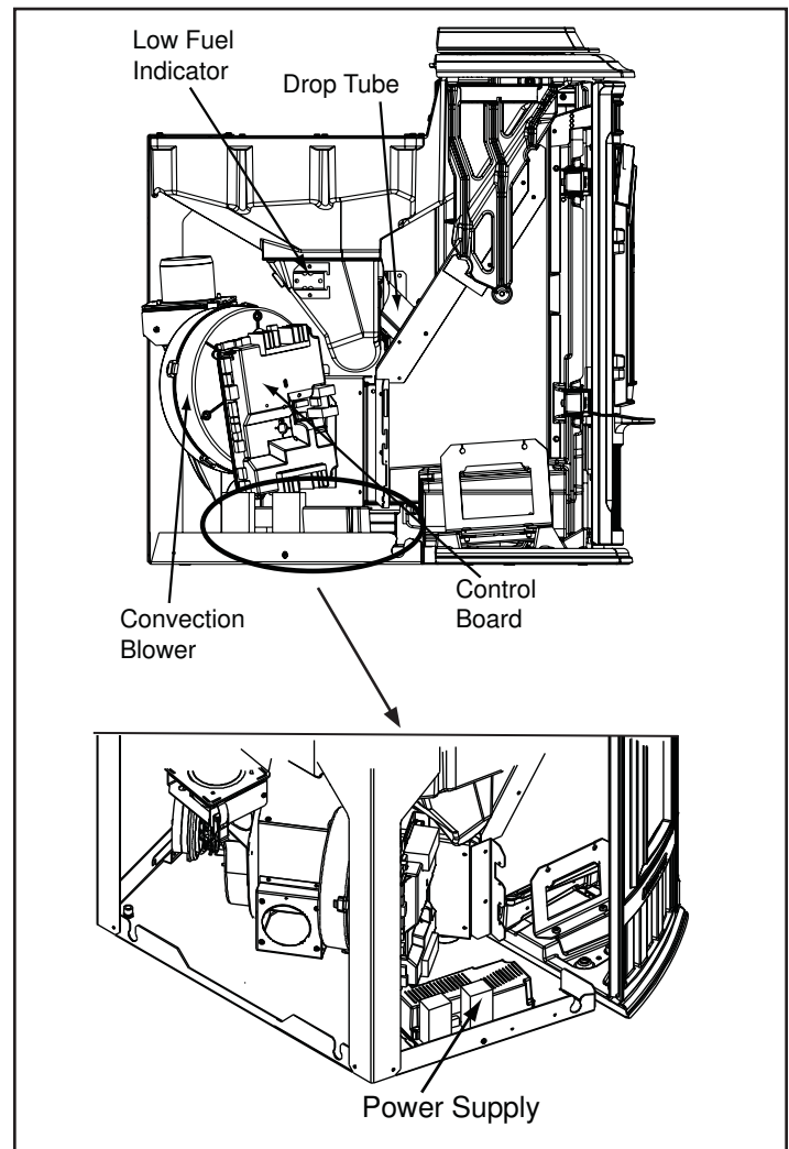
Figure 33.2 - Power Supply, Control Board, Convection Blower
