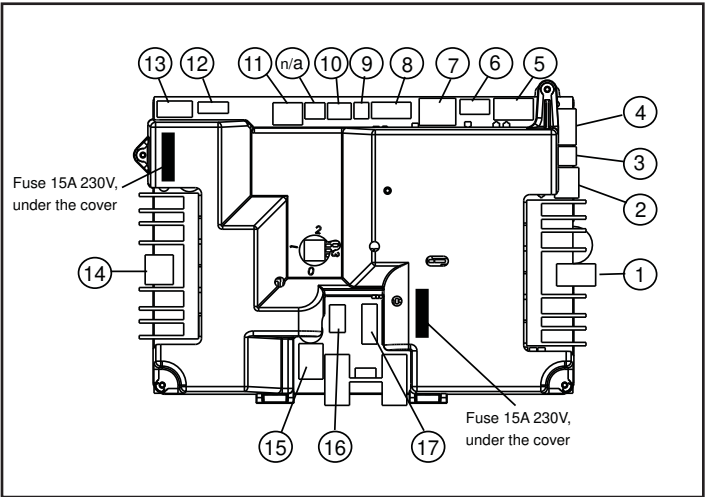
Figure 32.2 - Control Board
