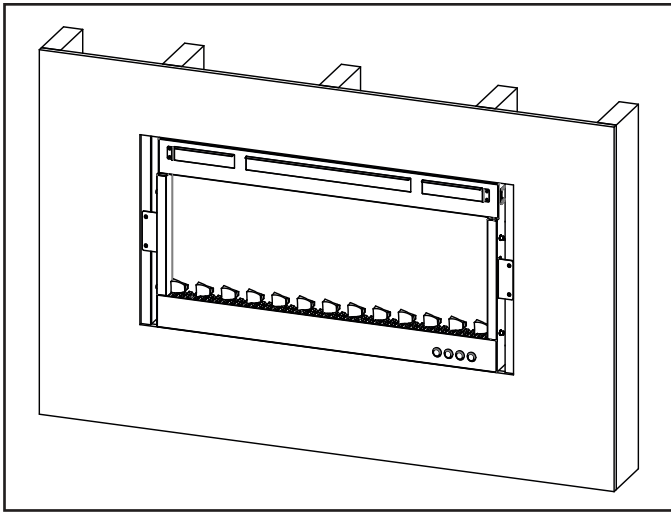
Figure 4.15 Stone Installation
