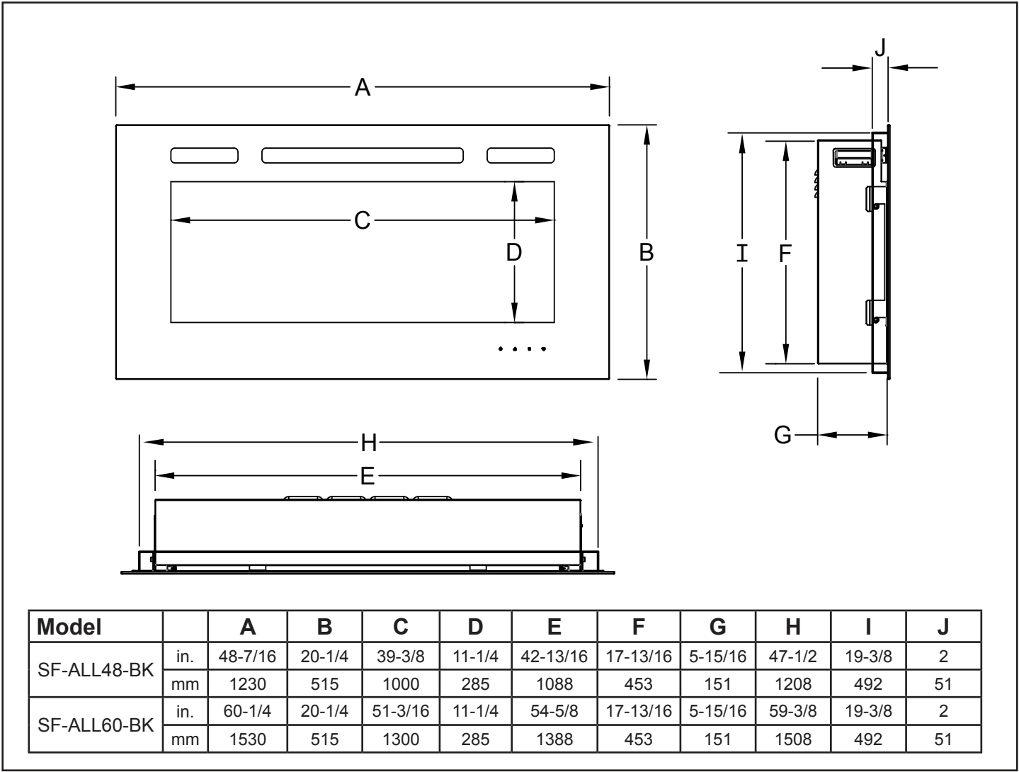
Figure 3.1 Appliance Dimensions
