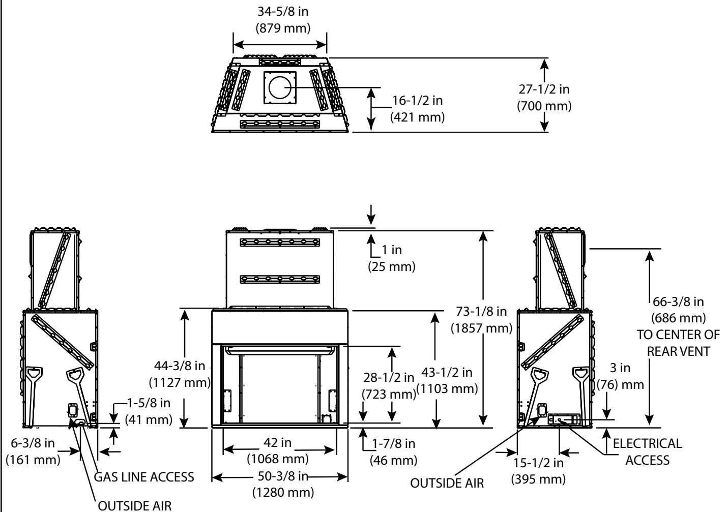
Figure 3.1 Appliance Dimensions
