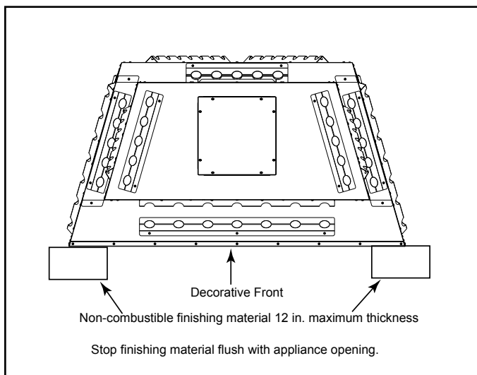
Figure 10.4 Non-Combustible Finishing Material (top and sides of appliance)
