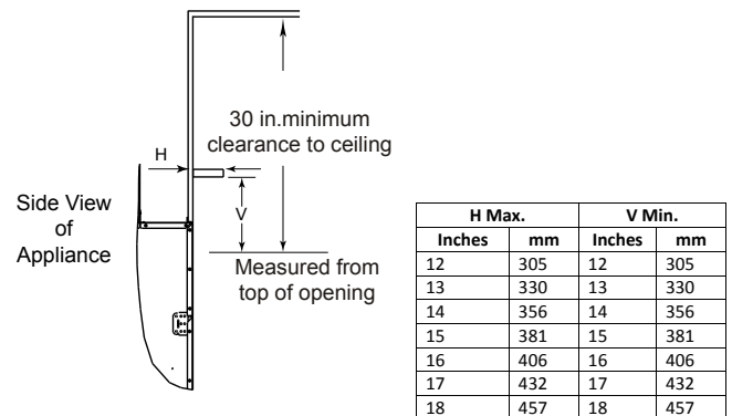
Figure 10.2 Minimum Vertical and Maximum Horizontal Dimensions of Combustibles
