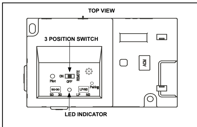
Figure 11.11 IFT-ECM
