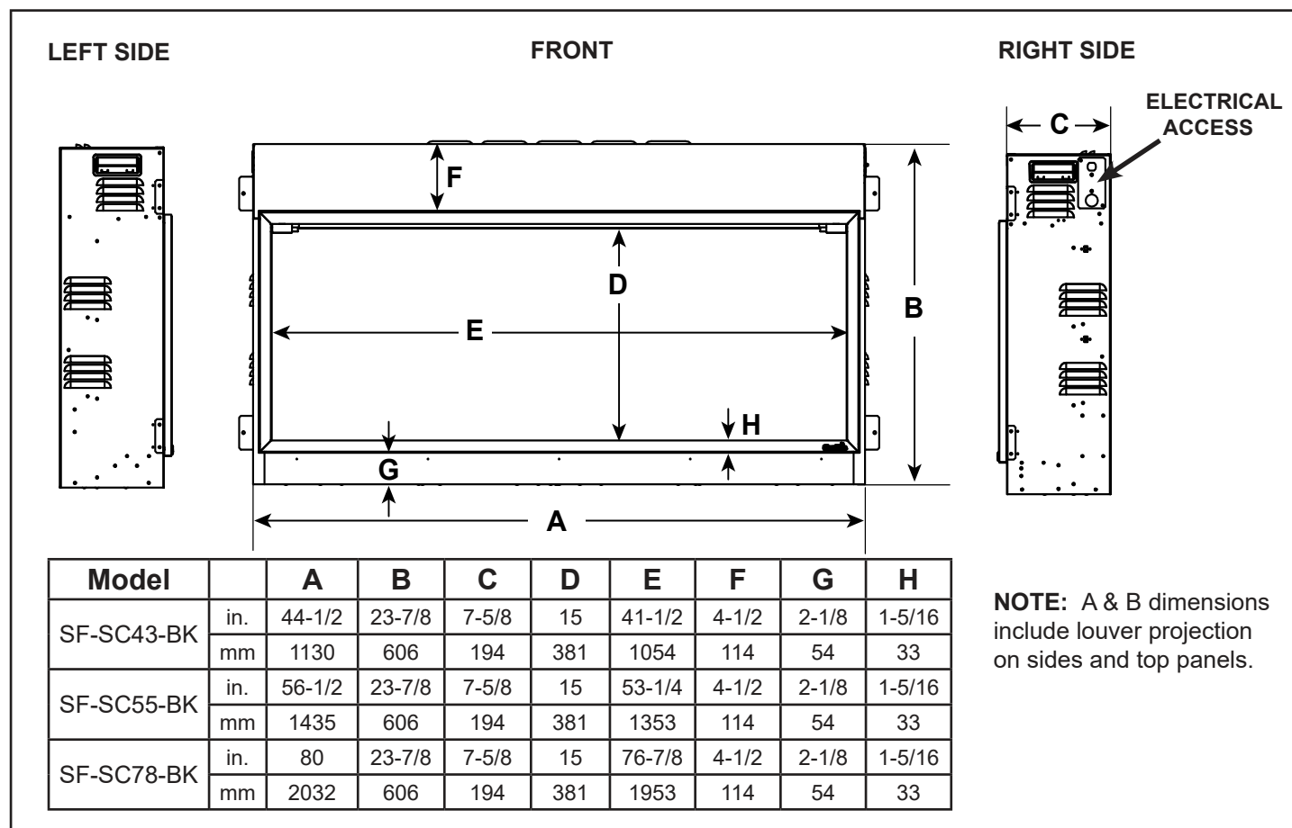
Figure 3.1 Appliance Dimensions
