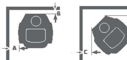
Stove parallel to wall
