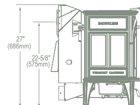
Side - Rear Vent
